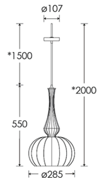
Dimensions in mm and approximate *Adjustable flex length
