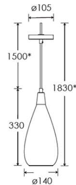
Dimensions in mm and approximate *Adjustable flex
